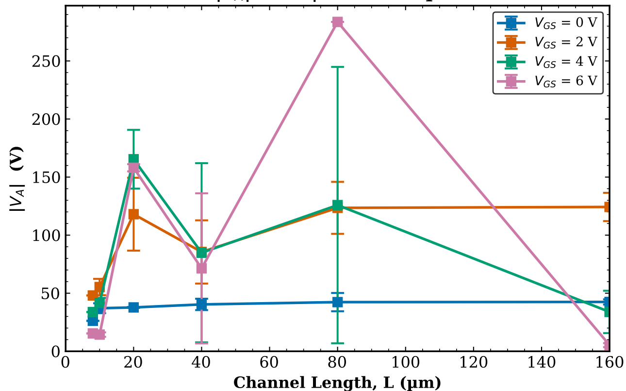
All Chips - Combined |V_A| vs L | W = 500\text{ }\mu\text{m}
